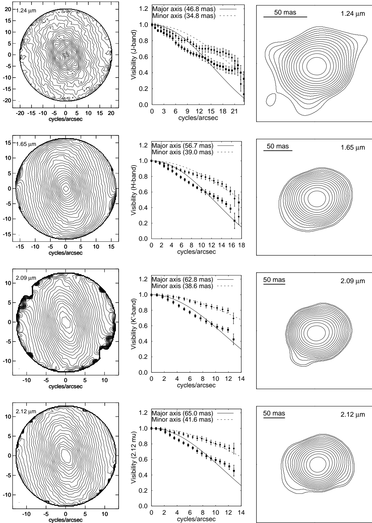
Fig. 1. Left column: two-dimensional visibilities. Middle column: cuts through the long and short axes of the visibilities and the visibilities of the best-fitting two-dimensional elliptical uniform-disk models fitted up to the telescope cut-off frequency. Right column: images of MWC 349A reconstructed by bispectrum speckle interferometry. The contours are plotted in steps of 0.3 mag (from 0.3 mag to 4.2 mag of peak intensity).
