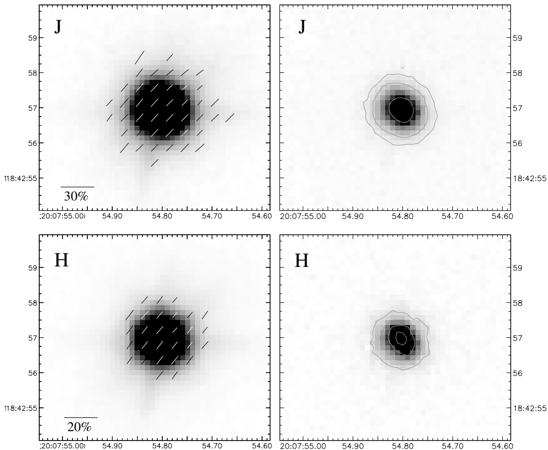
Figure 12. Polarimetric observations of IRAS 20056+1834 in the J and H bands. Details are as for Fig. 1.
