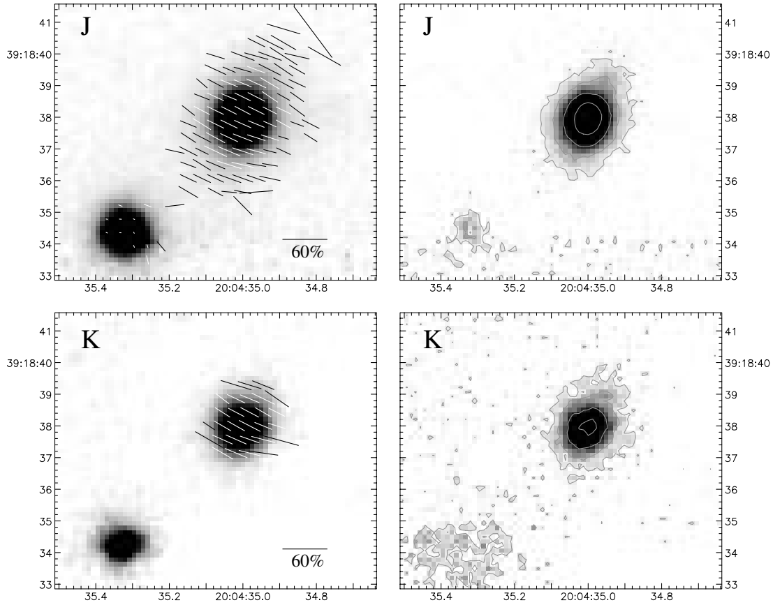
Figure 11. Polarimetric observations of IRAS 20028+3910 in the J and K bands. Details are as for Fig. 1.
