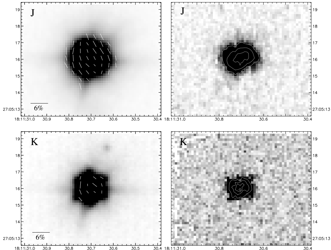
Figure 4. Polarimetric observations of IRAS 18095+2704 in the J and K bands. Details as for Fig. 1.
