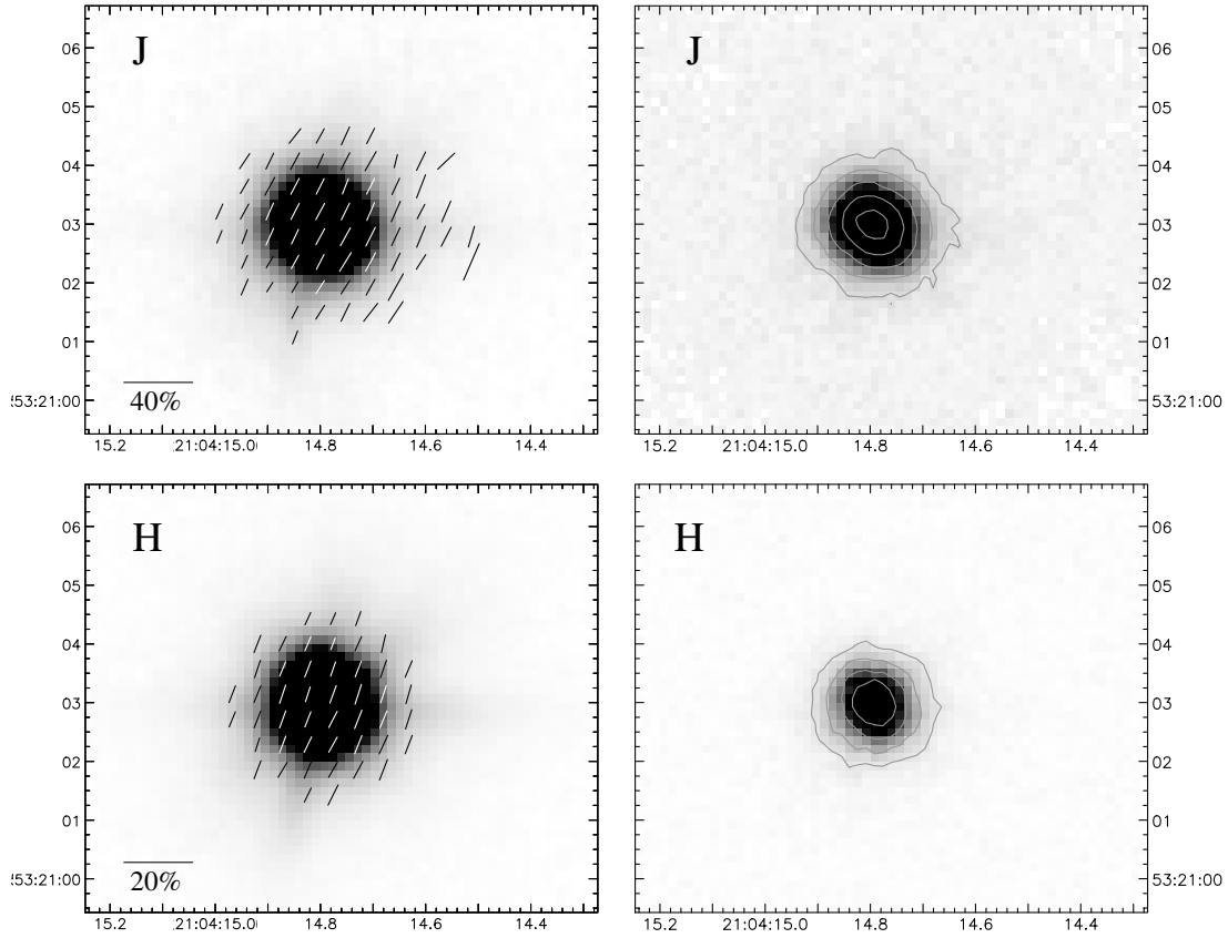
Figure 13. Polarimetric observations of IRAS 21027+5309 in J and H bands. Details are as for Fig. 1.
