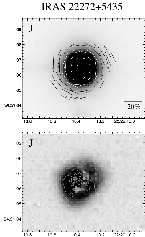
Figure 15. Polarimetric observations of IRAS 22272+5435 in the J band. The polarized flux contours are spaced logarithmically at intervals of 0.5 mag. Other details are as for Fig. 2.
