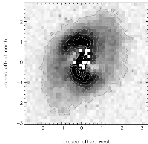
Figure 16. A close-up view of the CSE of IRAS 19475+3119 seen in scattered light (polarized flux) in the J band. Selected contours, spaced linearly, are superimposed on the grey-scale image to highlight the spiral arm structure. The single central contour is at 75 per cent of the total flux peak and marks the position of the stellar centroid. The line drawn between the two polarized flux peaks is 1.4 arcsec in length.
