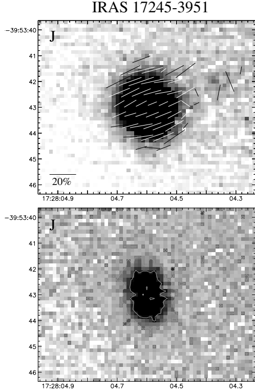
Figure 2. Polarimetric observations of IRAS 17245–3951 in the J band. The upper panel shows a grey-scale image of total flux superimposed with a linear polarization map (as described in Section 3.1.1). The lower panel shows a grey-scale image of polarized flux, with contours superimposed to highlight structure in the image. Other details are as in Fig. 1.
