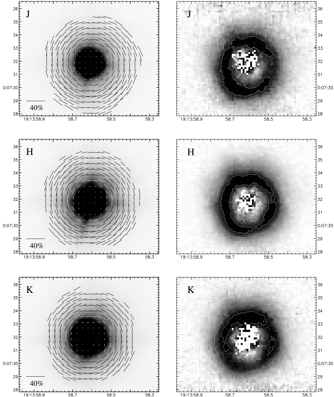
Figure 6. Polarimetric observations of IRAS 19114+0002 in the J , H and K bands. The polarized flux contours are spaced logarithmically at intervals of 0.5 mag. Other details are as for Fig. 1, with the addition of the H -band observations.
