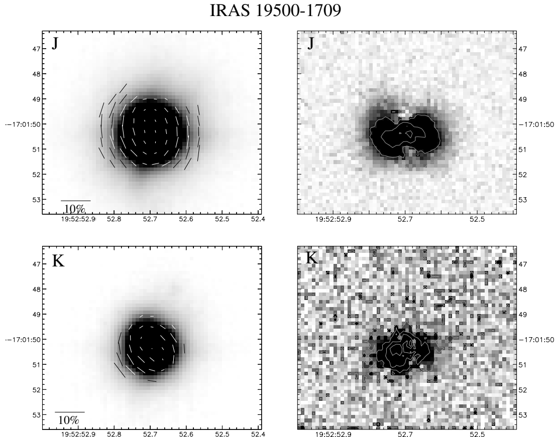
Figure 9. Polarimetric observations of IRAS 19500–1709 in the J and K bands. The polarized flux contours are spaced logarithmically at intervals of 0.8 mag. Other details are as for Fig. 1.
